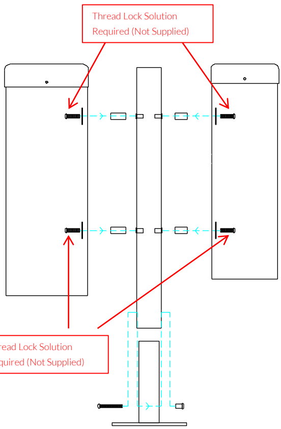
PPCONG FRONT
