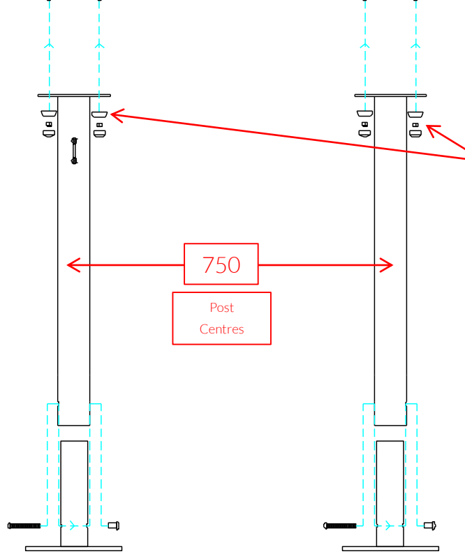
PPDUO FRONT
