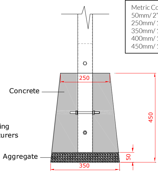
4 Fix instrument to Ground fix post using M10 bolt and Barrel Nut and use thread locking solution to prevent fixings working loose.
