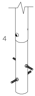
4 Fix instrument to Ground fix post using M10 bolt and Barrel Nut and use thread locking solution to prevent fixings working loose.
